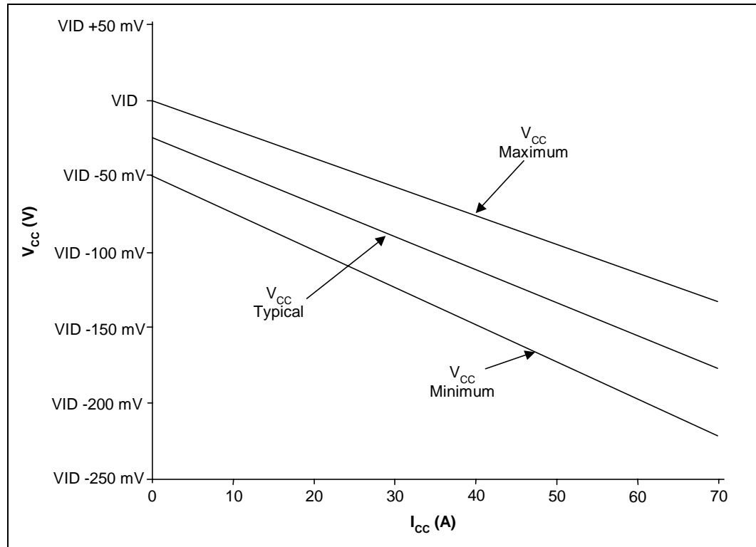
Figure 2-4. V_{CC} Static and Transient Tolerance (For Intel® Pentium® 4 Processor With 512-KB L2 Cache on 0.13 Micron Process)
