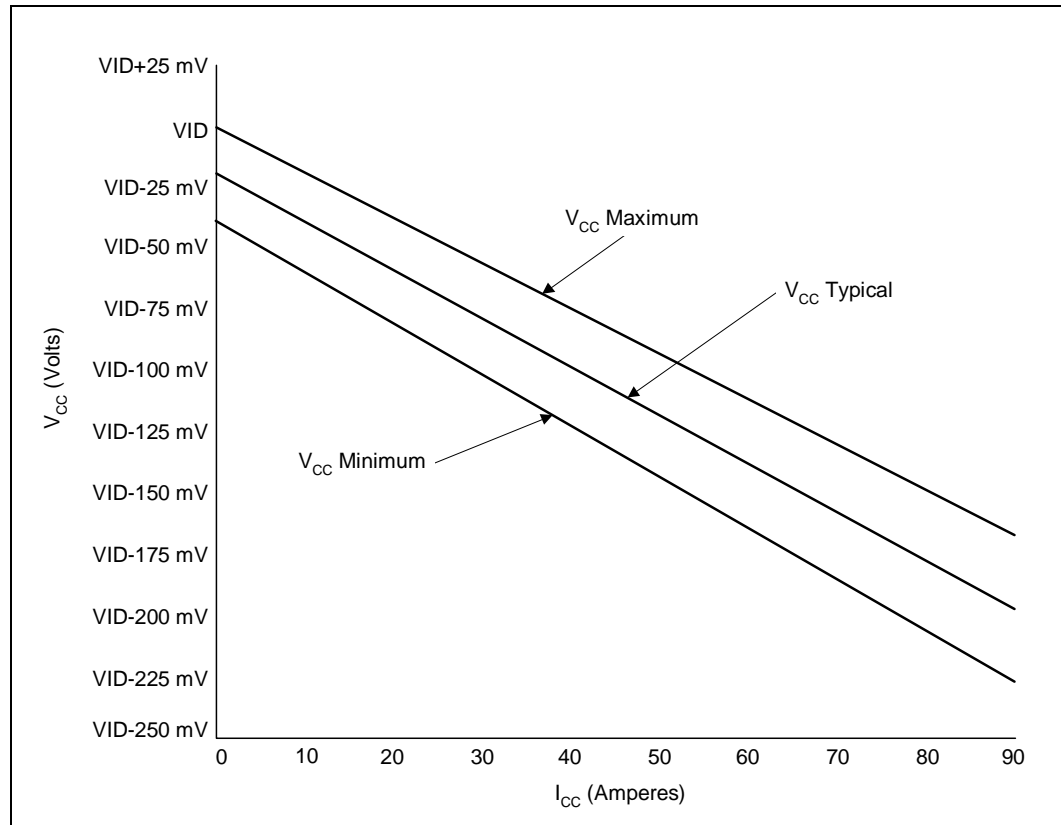
Figure 2-5. V_{CC} Static and Transient Tolerance (For Intel® Pentium® 4 Processor Extreme Edition Supporting Hyper-Threading Technology)
