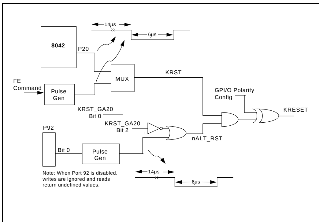
FIGURE 6 - KRESET GENERATION
