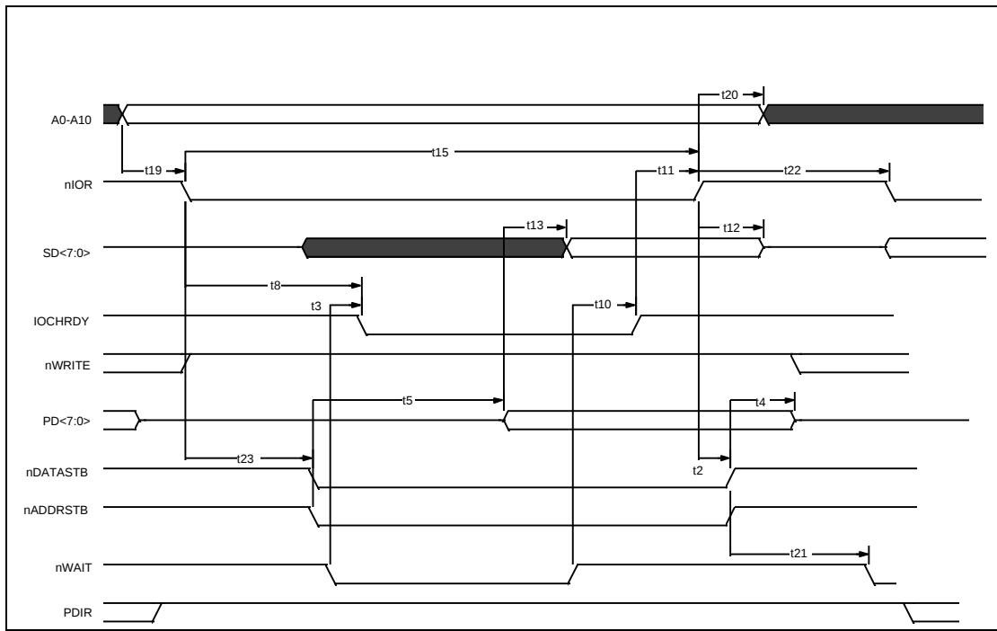
FIGURE 28A - EPP 1.7 DATA OR ADDRESS READ CYCLE
