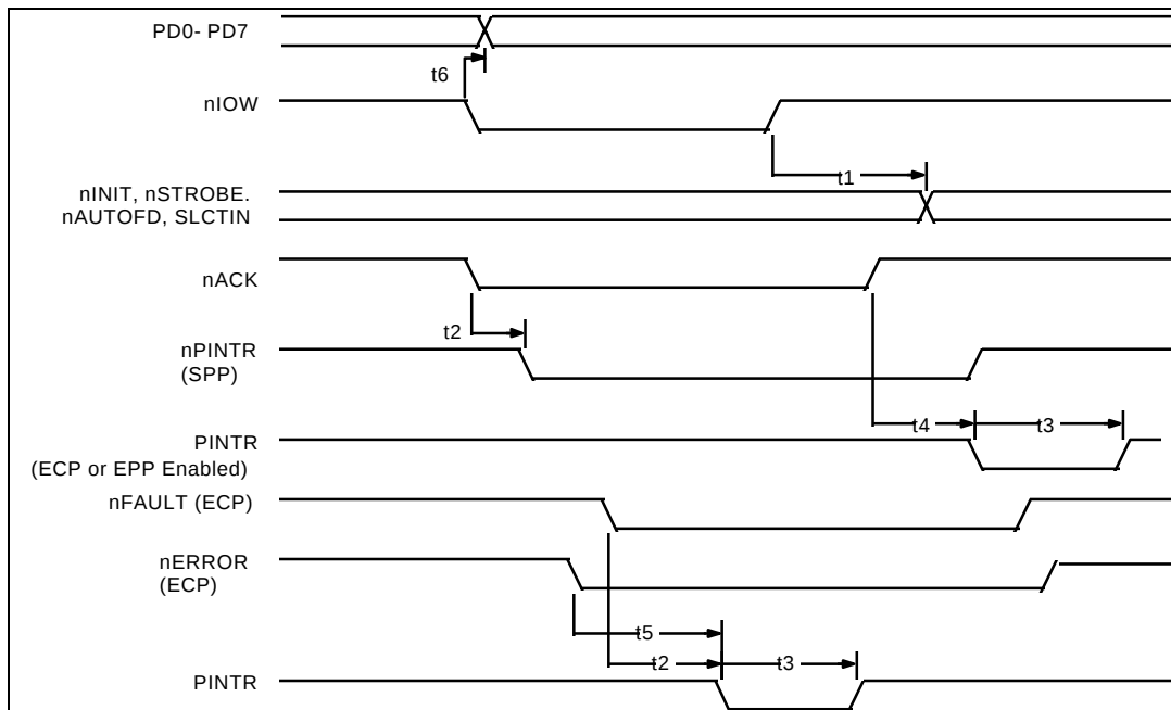
FIGURE 24 - PARALLEL PORT TIMING
