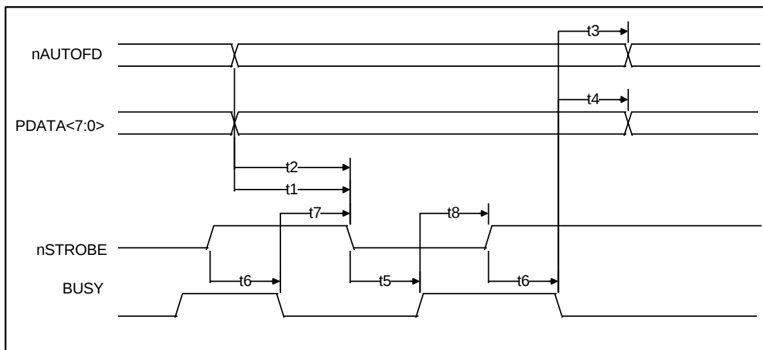
FIGURE 30 - ECP PARALLEL PORT FORWARD TIMING
