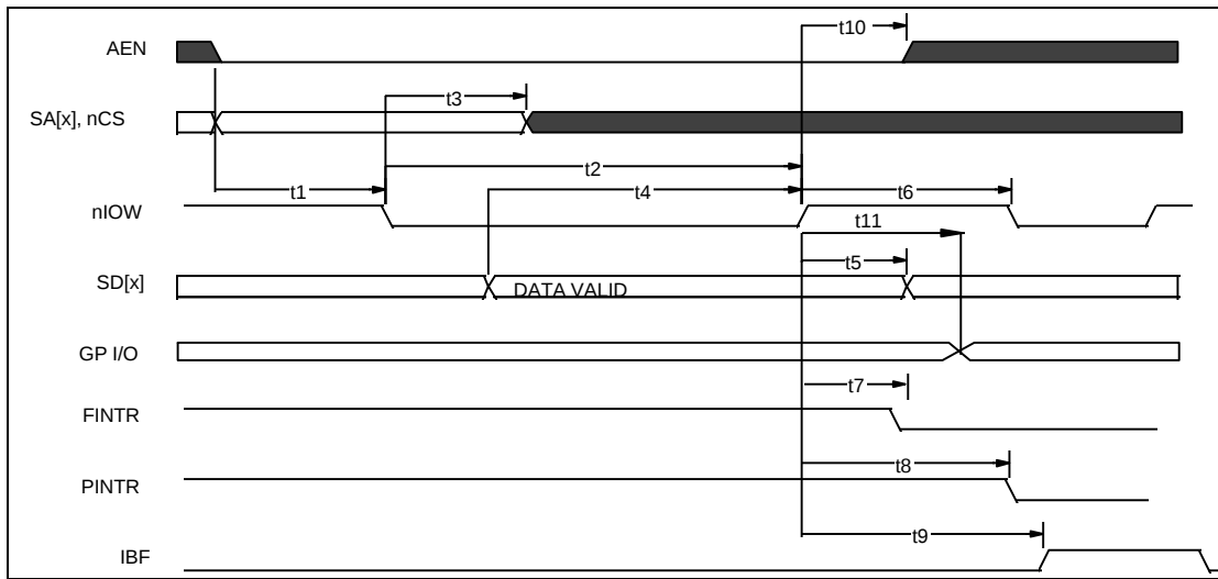
FIGURE 13 - ISA WRITE
