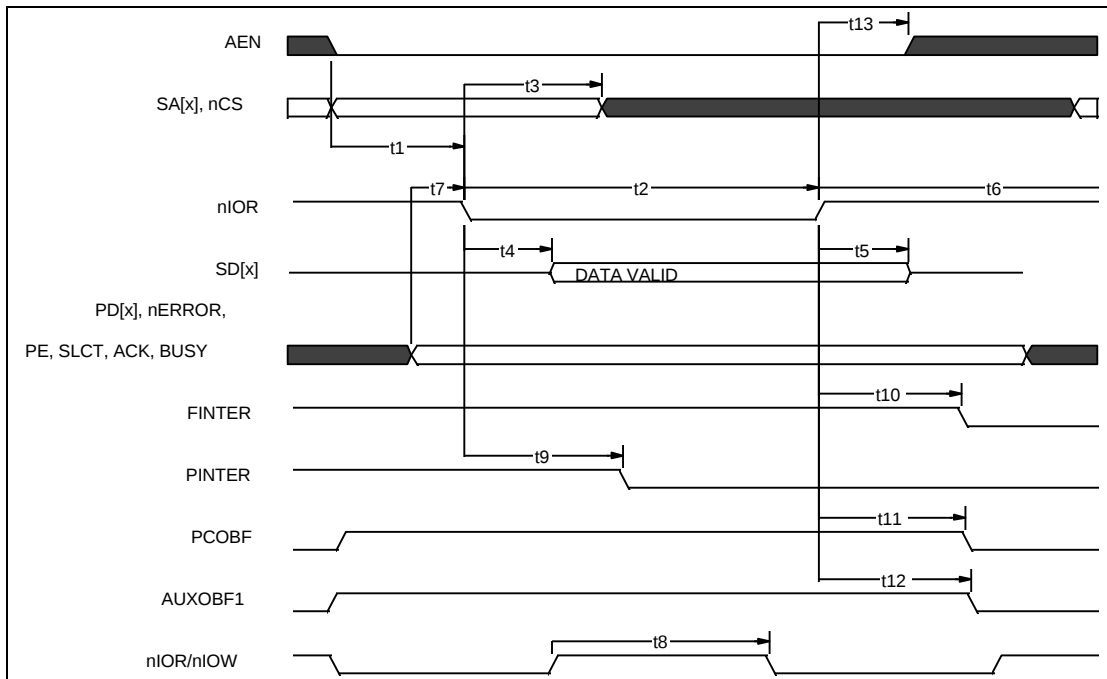
FIGURE 14 - ISA READ
