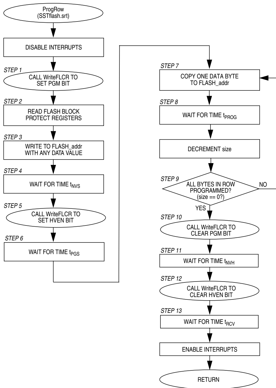
Figure 18. Subroutine ProgRow Flowchart
