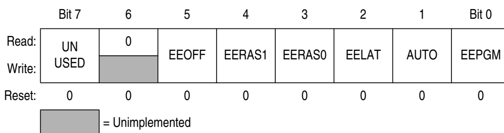
Figure 10. EEPROM Control Register (EExCR)
