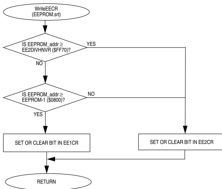
Figure 27. Subroutine WriteEECR Flowchart
