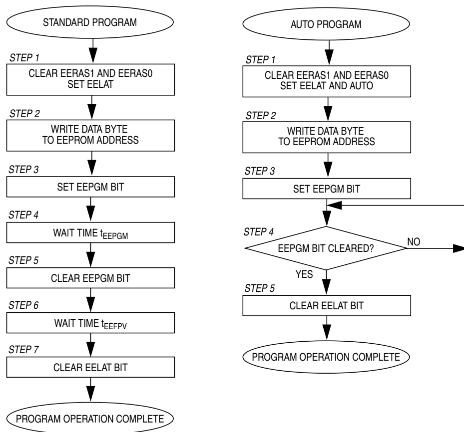
Figure 14. EEPROM Programming Algorithm Flowcharts
