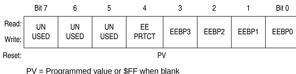
Figure 11. EEPROM Nonvolatile Register (EExNVR)
