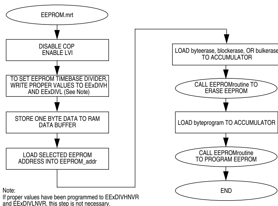
Figure 21. Standard EEPROM Main Routine Flowchart
