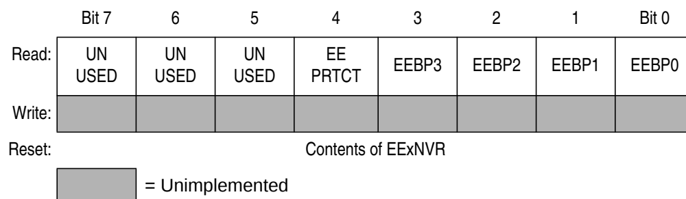
Figure 12. EEPROM Array Configuration Register (EExACR)
