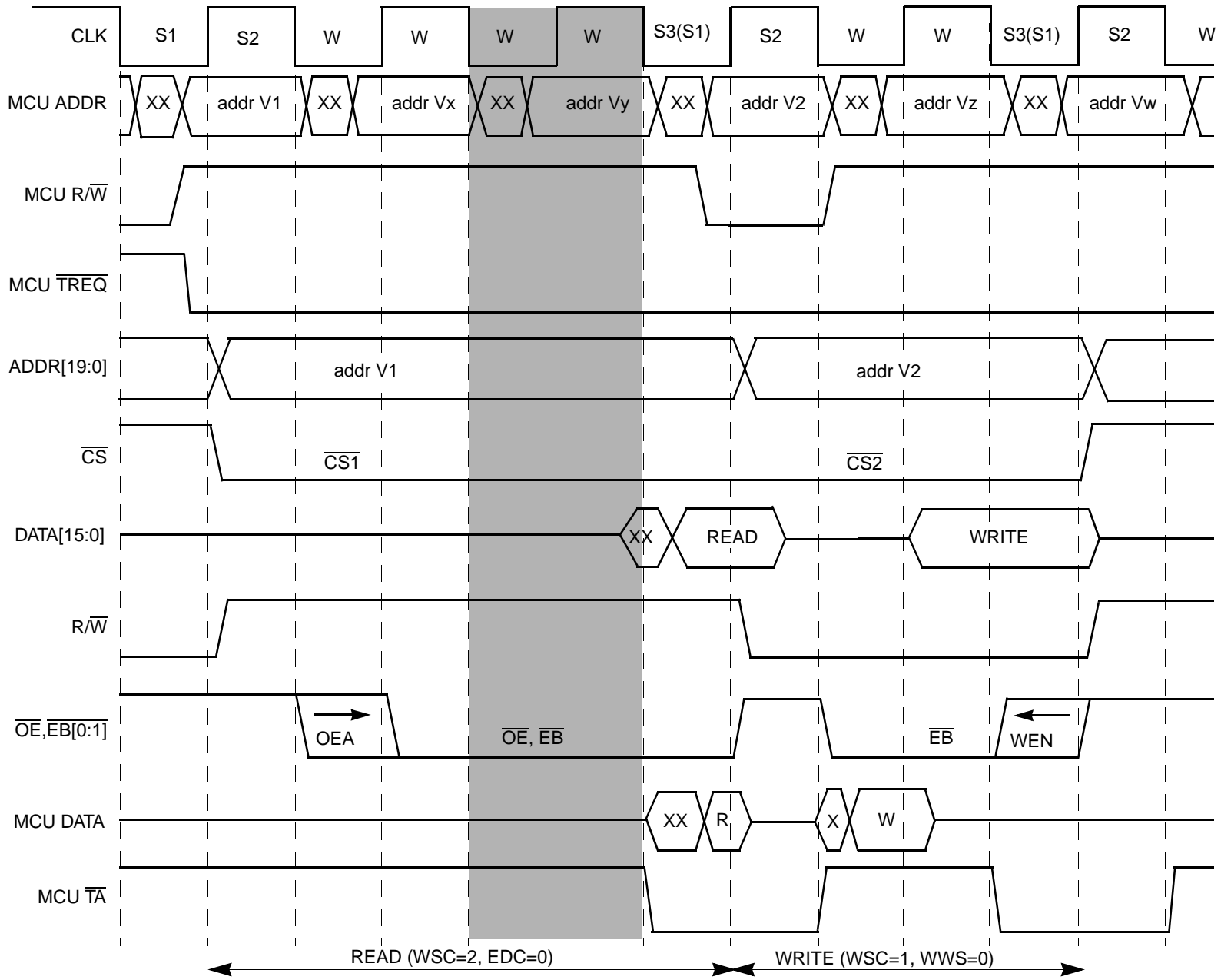
Figure 7-10 Write after Read Memory Access (CSA = 0, WSC = 2, EDC = 0)
