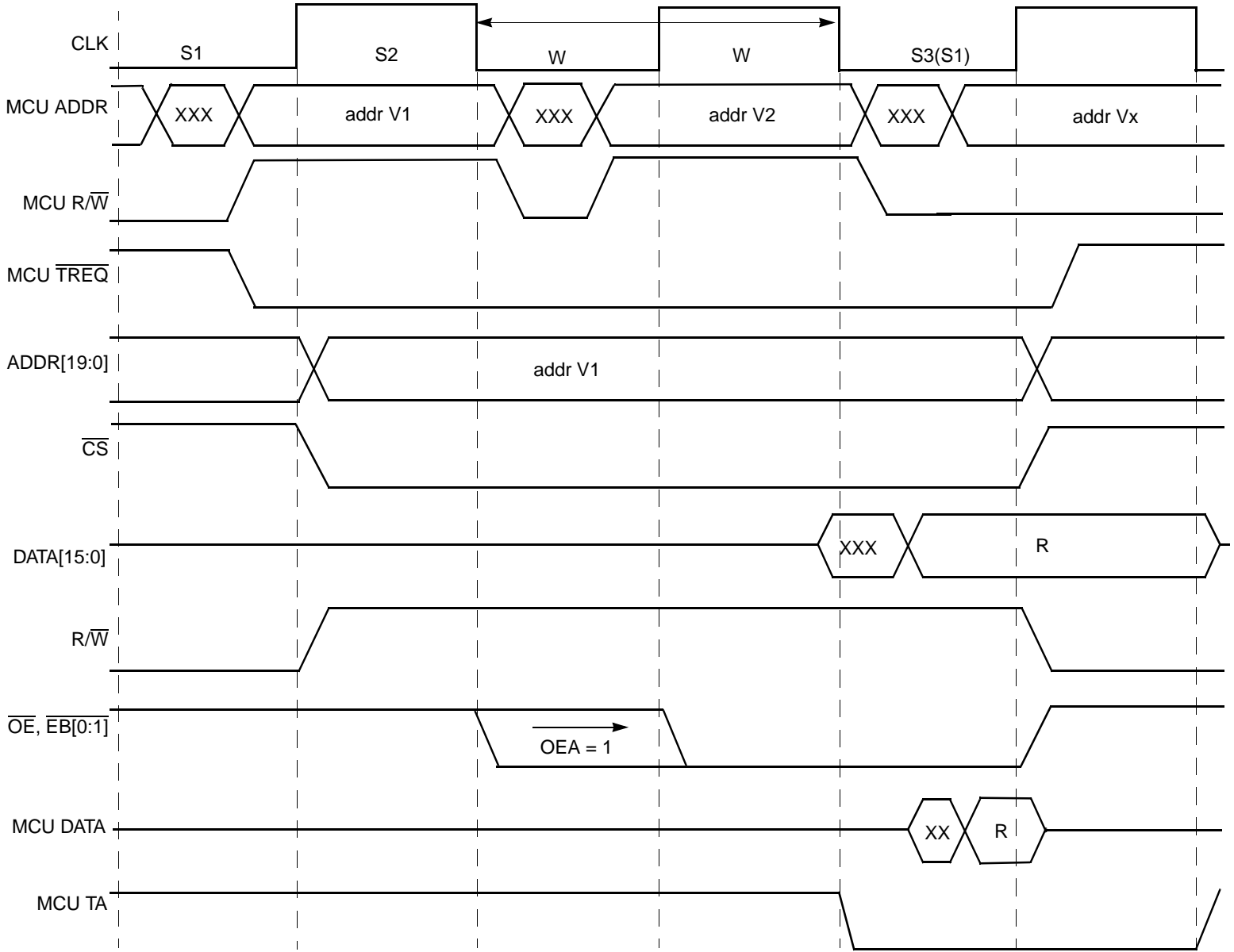
Figure 7-6 Read Memory Access (CSA = 0, WSC = 1)
